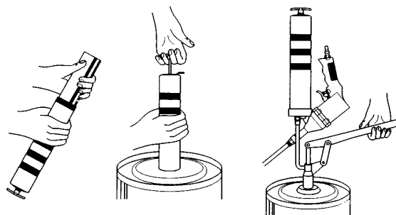
Cartridge Loading
